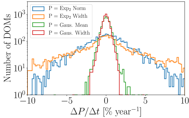
Figure 10. The change in the individual DOM fitted parameters from IceCube season IC86.2011 to IC86.2016. The histogram represents the rate of change, per IceCube season, of the fitted parameter labelled in the legend.
