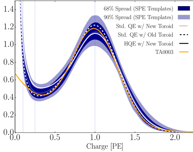
Figure 9. The inner (outer) dark blue region shows the 68% (90%) spread in the SPE charge templates for a given charge. Superimposed are the average SPE charge templates for the variety of hardware configurations shown in white. The TA0003 distribution, for comparison, is shown in orange. All curves have been normalized such that the area above 0.25 PE is the same.
