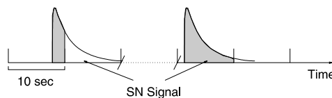
Fig. 6. The location of the time window of observation and the SN burst are uncorrelated, resulting in a reduced sensitivity.
