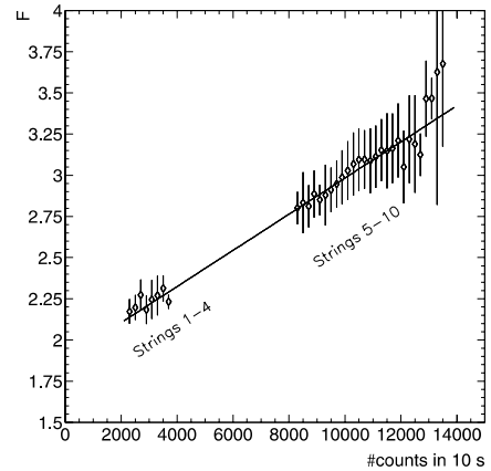
Fig. 4. F as a function of the noise, showing the strong correlation with the average of the measured rates. Note that the ordinate starts at F = 1.5 .
