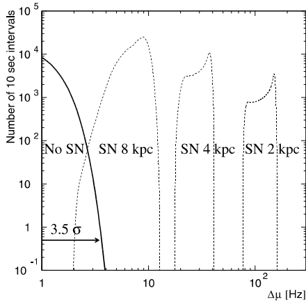
Fig. 9. Background distribution and expected SN signal of \Delta\mu for supernovae at different distances, in kpc. The smearing of the signal due to the fixed 10 s observation window is taken into account (see Fig. 6). Notice the logarithmic scale in \Delta\mu .
