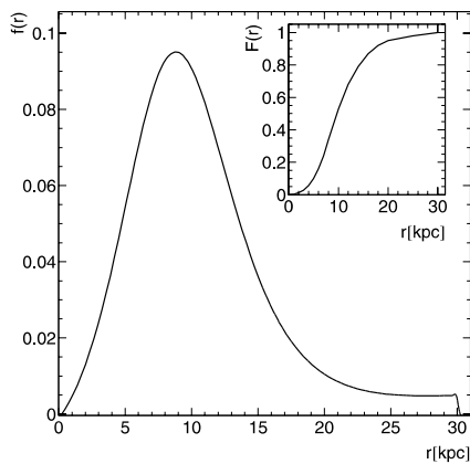
Fig. 1. The distribution f(r) of progenitor stars in the Milky Way, located within a distance r from the Earth. Inset: the corresponding cumulative distribution F(r) (taken from a model by Bahcall and coworkers [21,22]). The steep behavior around \sim 8 kpc is due to the high star density in the galactic bulge.
