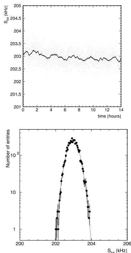
Fig. 5. Top: summed counting rate S_{tot} as a function of time for the selected OMs. The full line represents the MA. Bottom: the corresponding S_{tot} -distribution (dots) fitted with a Gaussian (curve).
