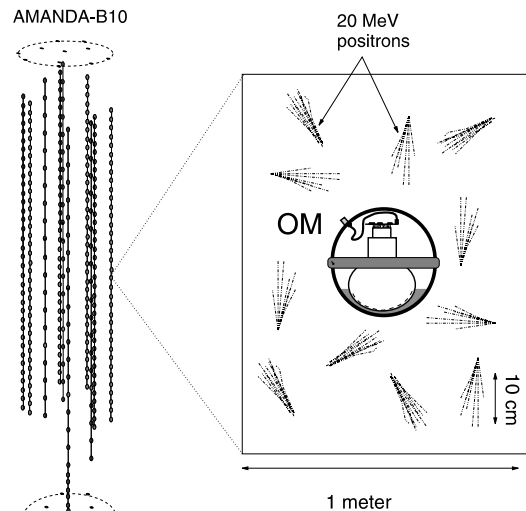
Fig. 2. View of the detector and of the expected positron tracks produced in CC \bar{\nu}_e interactions within AMANDA.
