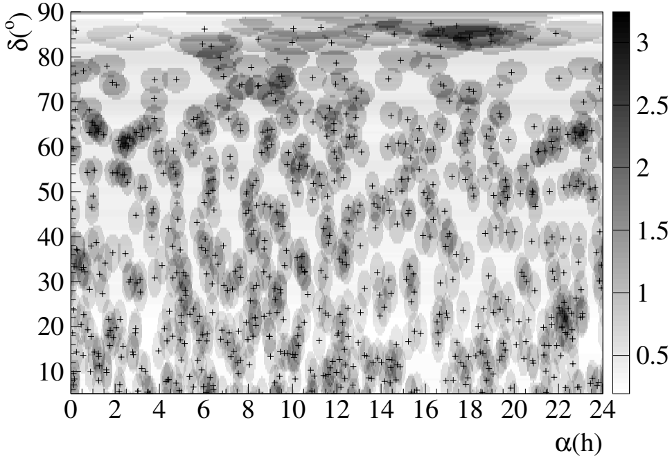
Fig. 2. Skymap of 646 neutrino events observed from arrival directions below the horizon at the south pole (i.e. from declination greater than zero degrees) in the 2000-02 point source analysis. These events are mostly atmospheric neutrinos and misreconstructed downgoing muons. No evidence for an excess of neutrinos above these backgrounds is present, leading to limits across the sky, and on individual sources. The gray-scale shows the value of the 90% upper limit across the sky, in units of E^2\Phi_{90} = 10^{-7} \text{ GeV cm}^{-1} \text{ sr}^{-1}
