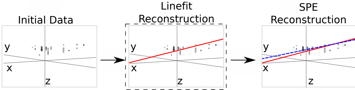
Fig. 2: The reconstruction pipeline used to process data in the IceCube detector. Each point indicates a PMT that recorded a photon (PMTs that recorded nothing are omitted). After initial data is collected and passed through some noise filters, the data is processed by a linefit (solid line), which is used as the seed for the SPE (dashed line). The SPE reconstruction is then evaluated as a potential neutrino. Our work in the reconstruction problem makes changes to the linefit reconstruction algorithm (indicated by the dashed box).
