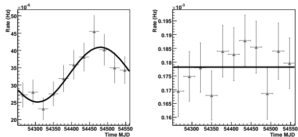
Fig. 3. Uptime corrected rates and their fits for the southern (left) and northern (right) skies.
