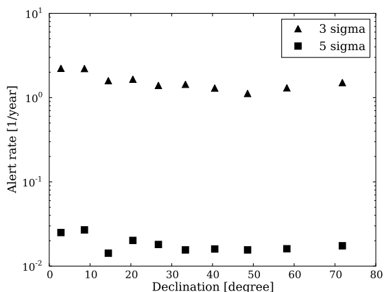
Fig. 4. Preliminary alert rate from atmospheric neutrino background for IceCube in its 2009/2010 configuration with 59 deployed strings for an alert threshold for the multiplet significance corresponding to 3\sigma (upper points) and 5\sigma (lower points) and a bin size of 2^\circ .
