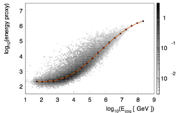
Fig. 6 The energy resolution for muons is approximately 0.3 in log(energy) over a wide energy range
