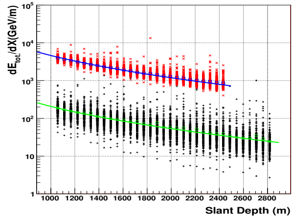
Fig. 2. Muon bundle energy loss as function as slant depth. Two examples are given in the figure: red x for vertical 1 EeV iron showers and the black + for 30 degree 50 PeV proton showers. Open squares and circles are the mean value of the Monte Carlo results for iron and proton showers. Eq. ( 5) is represented by the two curves.
