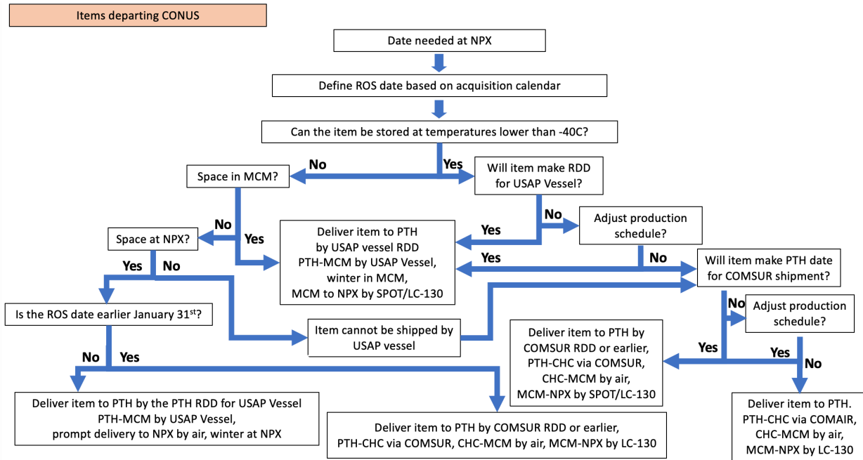
Figure 4: Shipping flowchart for point of departure within CONUS
