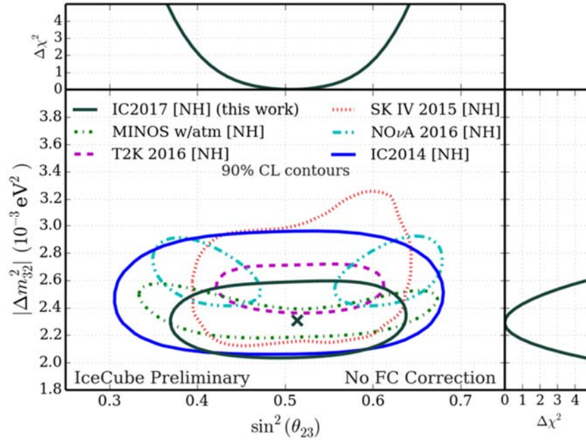
Figure 2.1-5: Oscillation parameters measured with three years of DeepCore data (2012-2014). The 90% confidence contours are shown in comparison with those of the most sensitive experiments. At the top and on the right side of the figure, the log-likelihood profiles for individual oscillation parameters are given. Normal mass hierarchy is assumed. The measured is performed in the energy range of 5-55 GeV, exceeding that of previous experiments by one order of magnitude.
