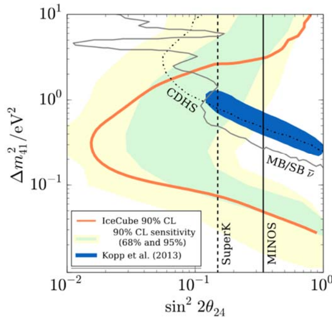
Figure 2.1-6: Results from the IceCube search for light sterile neutrinos using high-energy atmospheric neutrinos. The 90% (orange solid line) CL contour is shown with bands containing 68% (green) and 95% (yellow) of the 90% contours in simulated pseudo-experiments, respectively. The contours and bands are overlaid on 90% CL exclusions from previous experiments and the MiniBooNE/LSND 90% CL allowed region.
