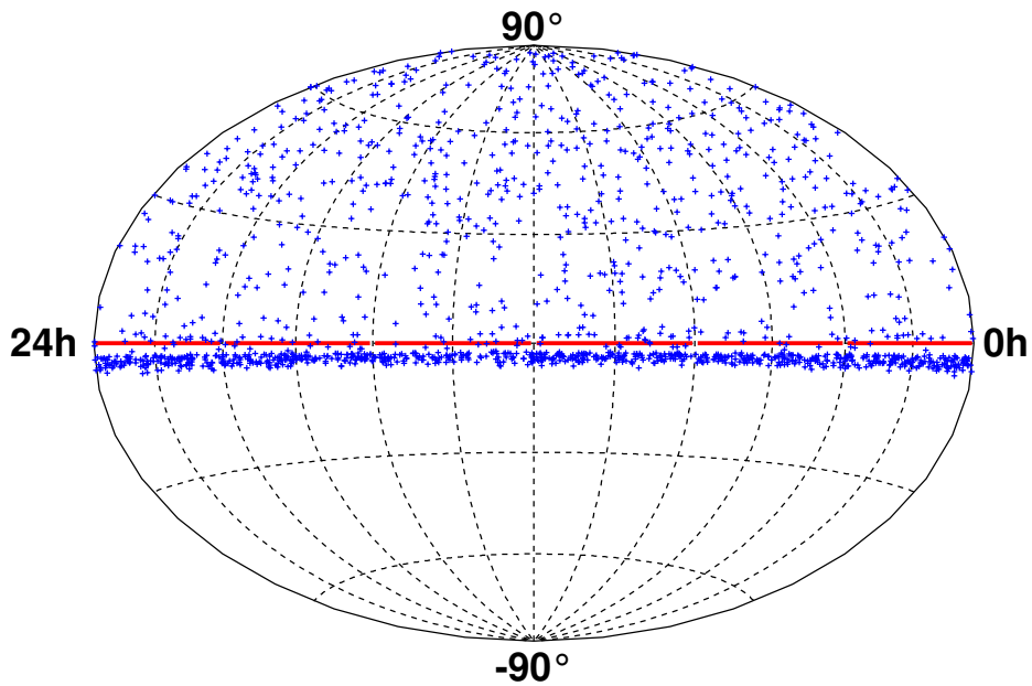
Fig. 1. Skymap of 699 neutrino events observed from arrival directions below the horizon at the south pole (i.e. from declination greater than zero degrees) in the 2000 point source analysis. These events are mostly atmospheric neutrinos and misreconstructed downgoing muons. No evidence for an excess of neutrinos above these backgrounds is present, leading to limits across the sky, and on individual sources.
